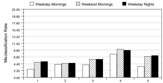
Figure 4: Misclassification Rates of Classifier Trained on First 10 Weekdays
