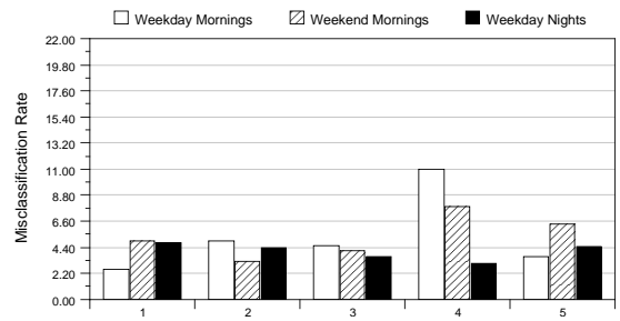
Figure 3: Misclassification Rates of Classifier Trained on First 8 Weekdays
